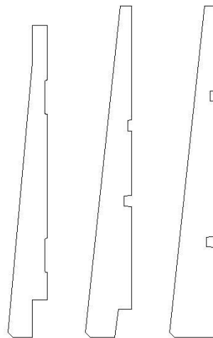
* 145X21 * 175X25X6 175X25X6 DRESSED FACE SAWN FACE SAWN FACE REBATED REBATED
